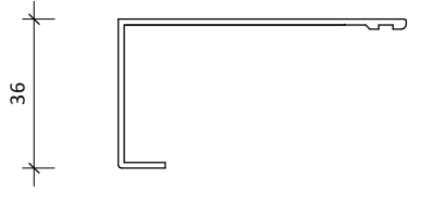
RKFL-15 powder coated aluminium jamb flashing. Colour to suit joinery
