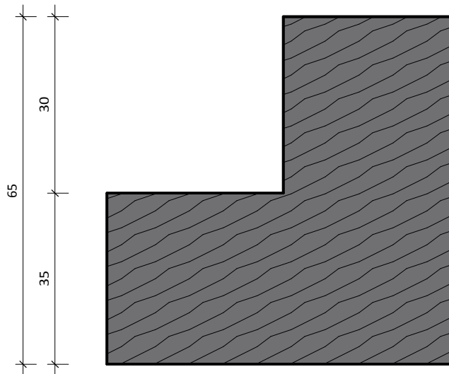
65x65x35mm External timber moulding
